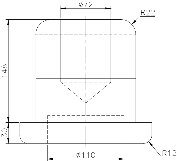
FRONT SCALE 1/3
