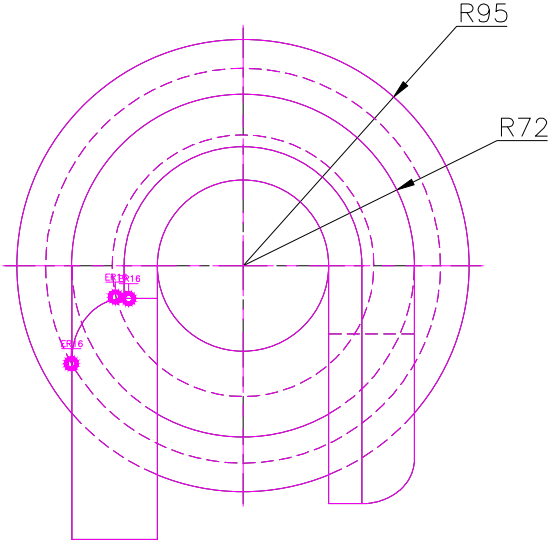
TOP SCALE 1/3
