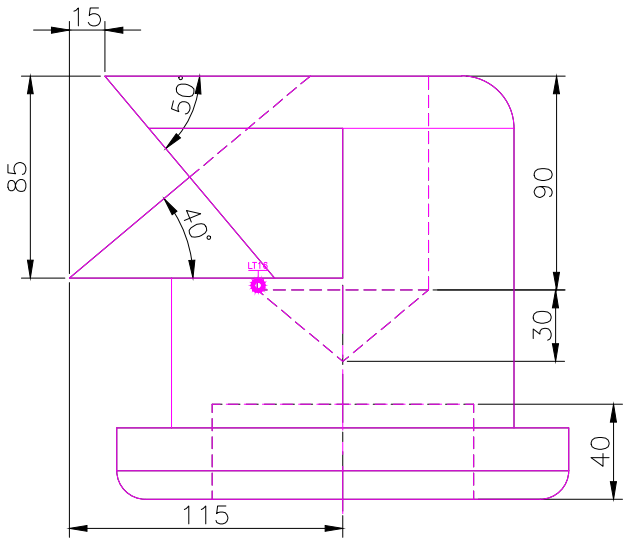
RIGHT SCALE 1/3
