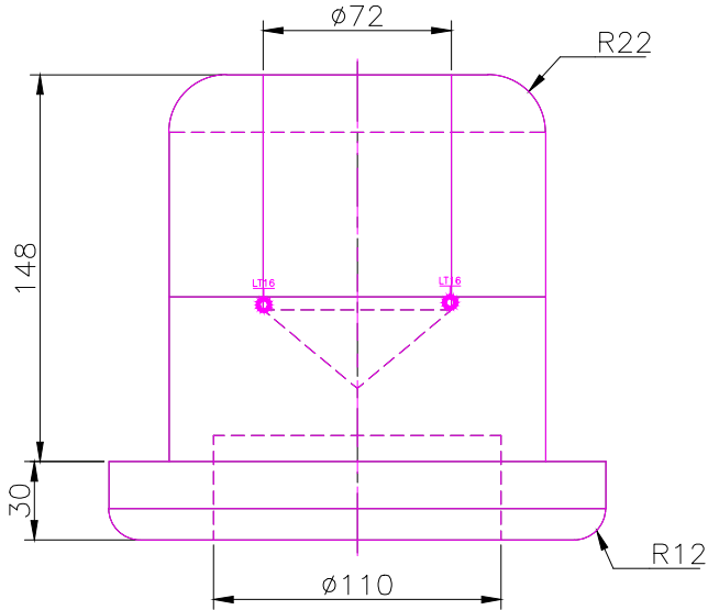
FRONT SCALE 1/3
