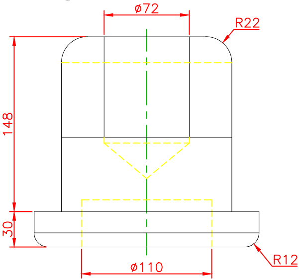
FRONT SCALE 1/3
