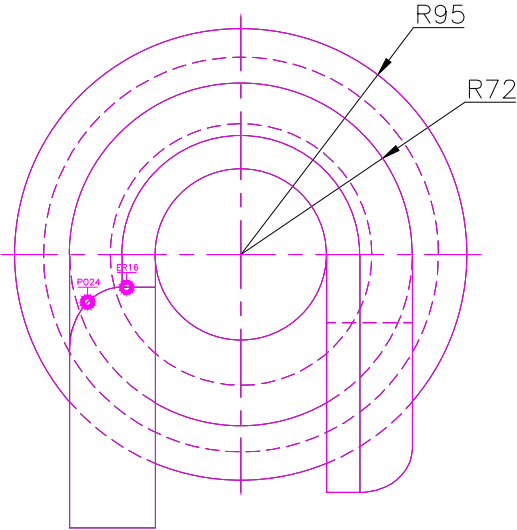
TOP SCALE 1/3
