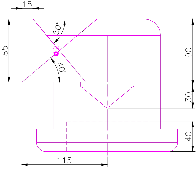
RIGHT SCALE 1/3
