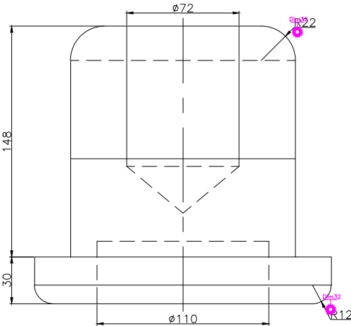
FRONT SCALE 1/3
