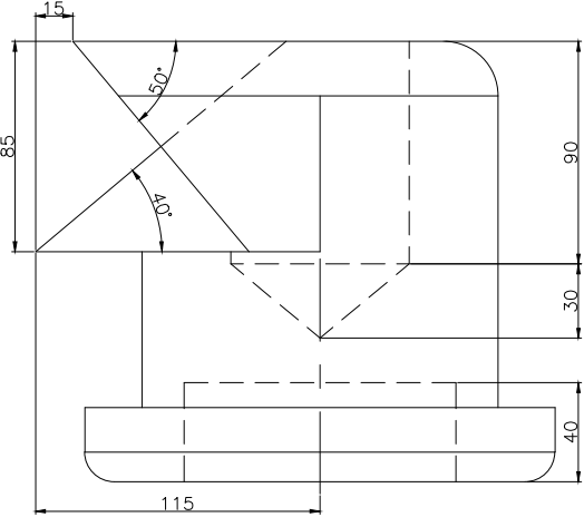
RIGHT SCALE 1/3
