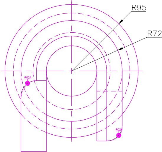
TOP SCALE 1/3
