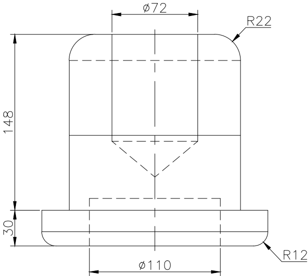
FRONT SCALE 1/3
