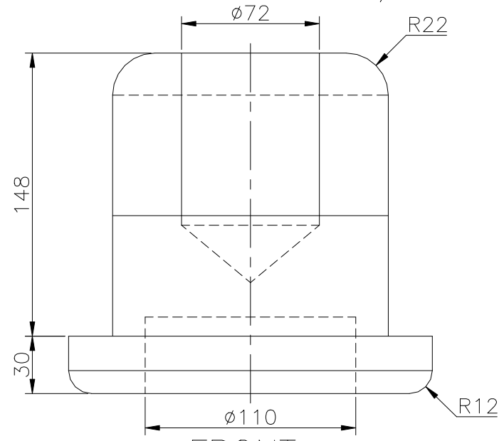
FRONT SCALE 1/3
