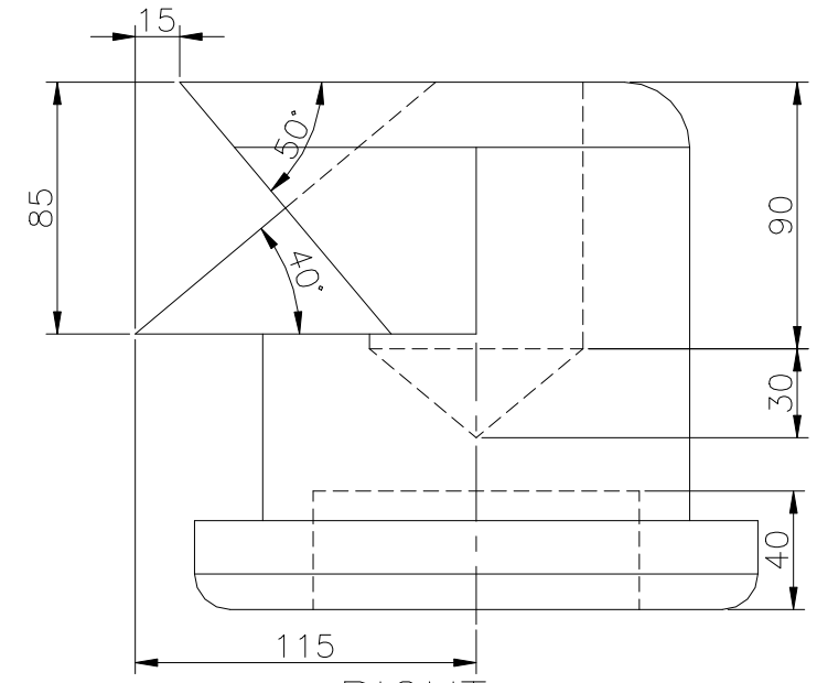
RIGHT SCALE 1/3
