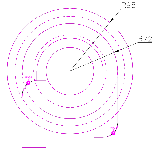
TOP SCALE 1/3
