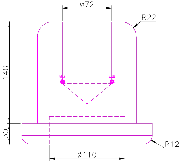
FRONT SCALE 1/3
