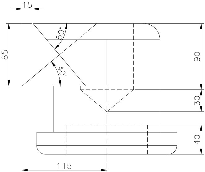
RIGHT SCALE 1/3
