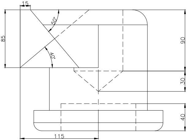
RIGHT SCALE 1/3
