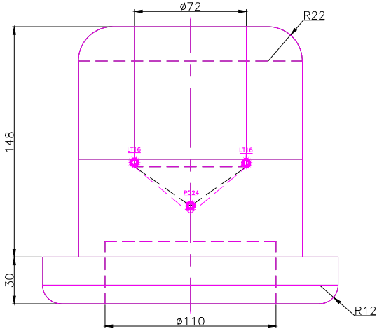
FRONT SCALE 1/3
