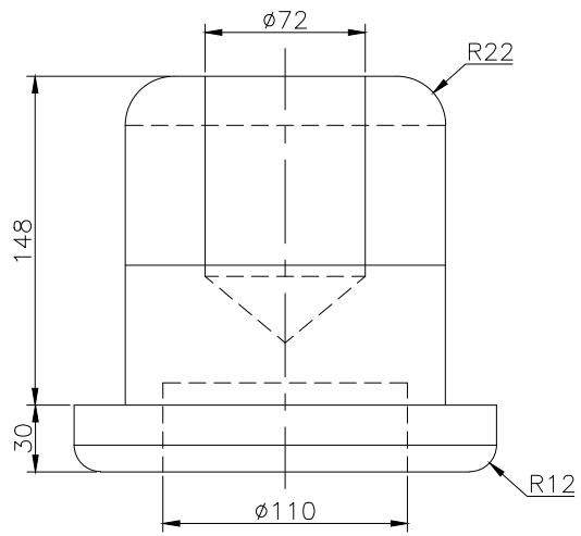
FRONT SCALE 1/3
