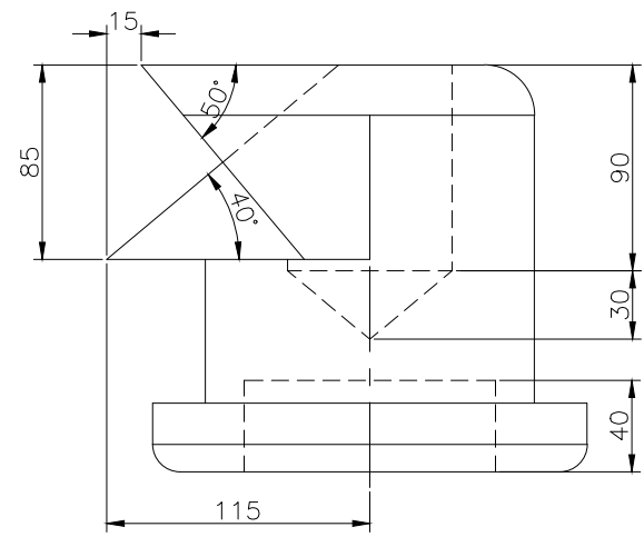
RIGHT SCALE 1/3
