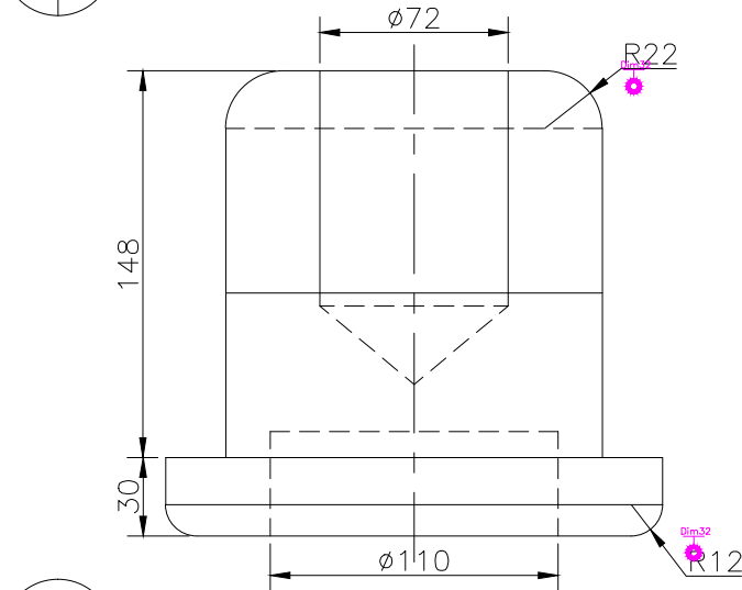
FRONT SCALE 1/3
