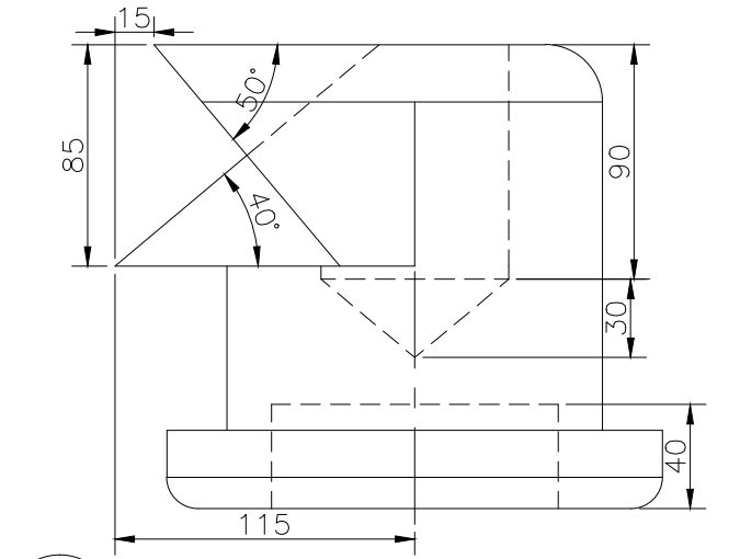
RIGHT SCALE 1/3
