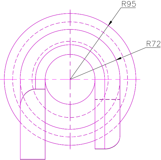
TOP SCALE 1/3
