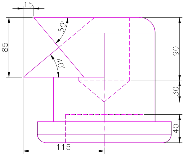
RIGHT SCALE 1/3
