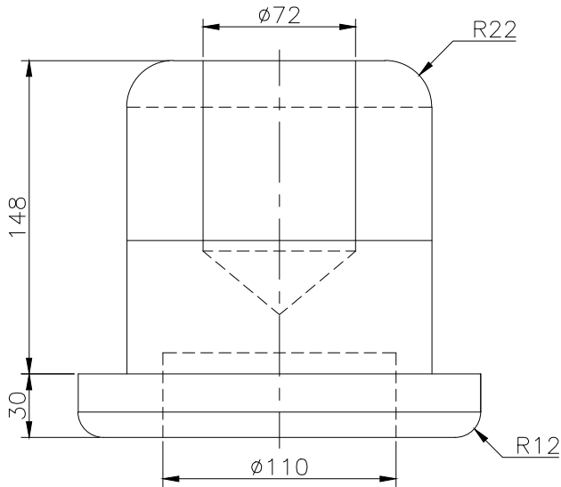
FRONT SCALE 1/3
