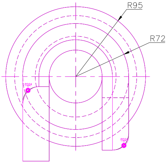
TOP SCALE 1/3
