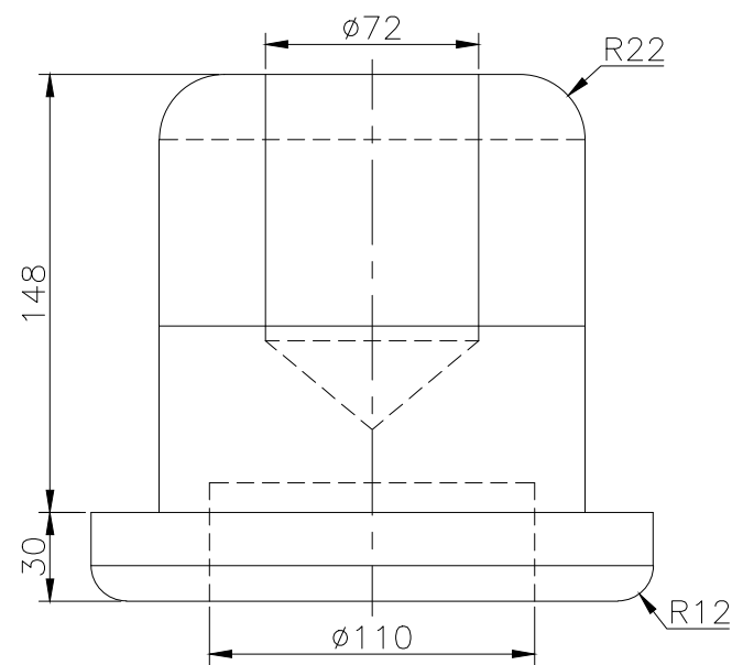
FRONT SCALE 1/3
