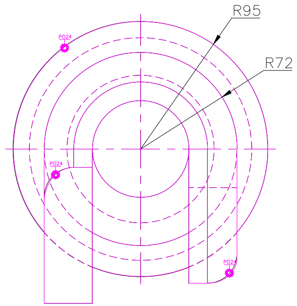
TOP SCALE 1/3
