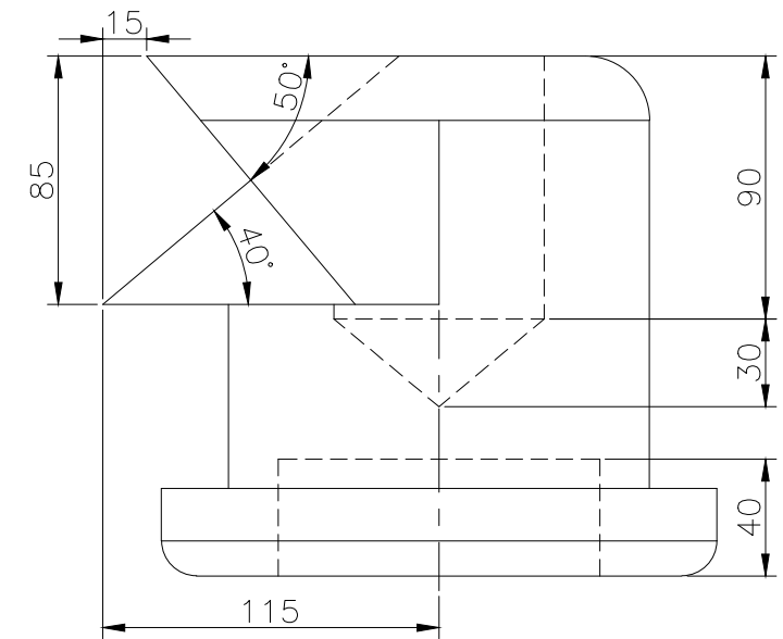
RIGHT SCALE 1/3
