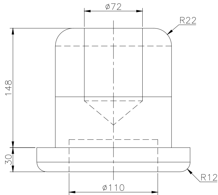
FRONT SCALE 1/3
