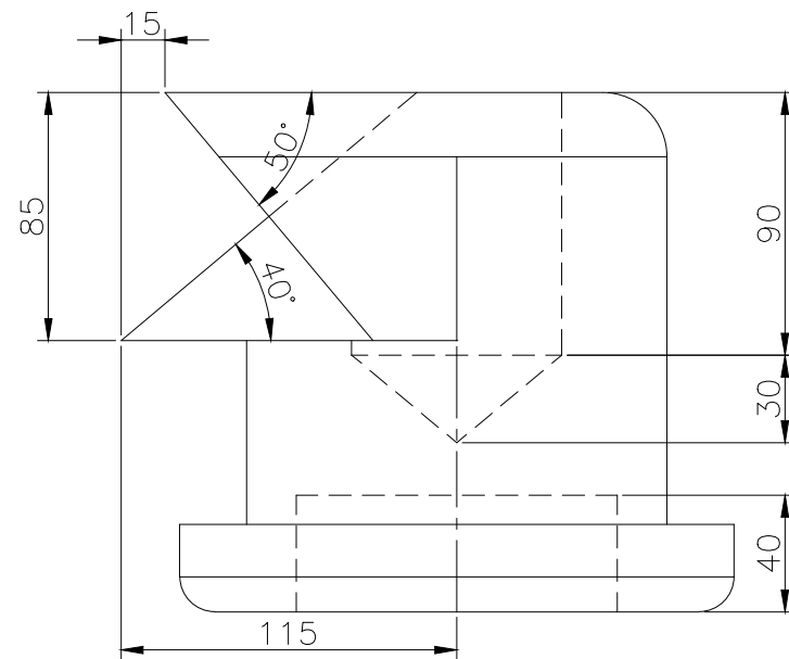
RIGHT SCALE 1/3
