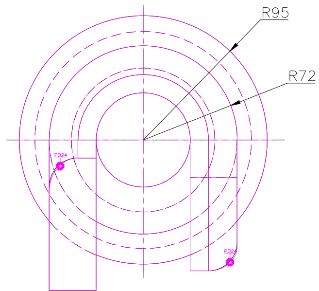
TOP SCALE 1/3
