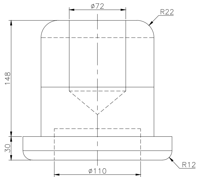
FRONT SCALE 1/3
