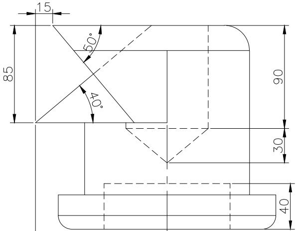
RIGHT SCALE 1/3
