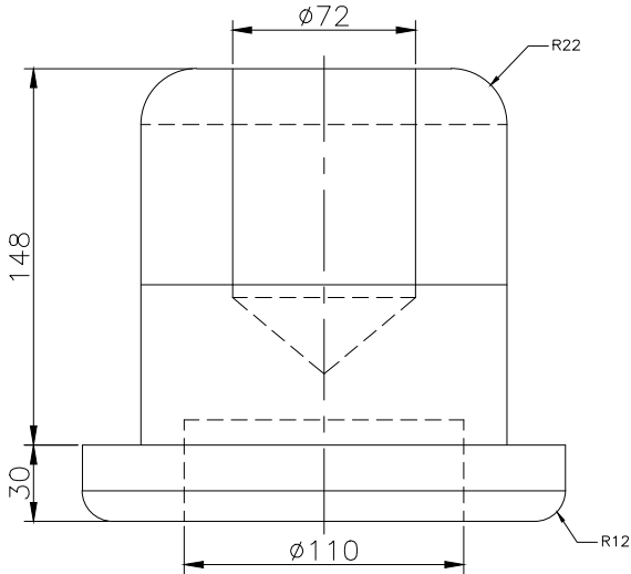
FRONT SCALE 1/3
