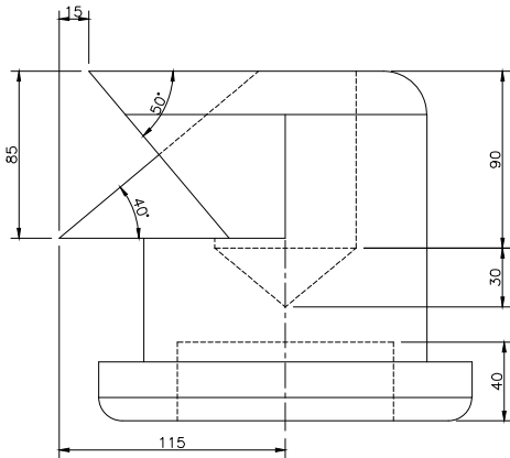
RIGHT SCALE 1/3
