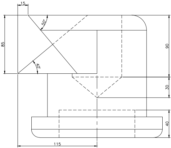
RIGHT SCALE 1/3
