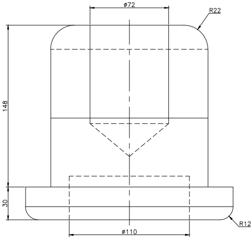
FRONT SCALE 1/3
