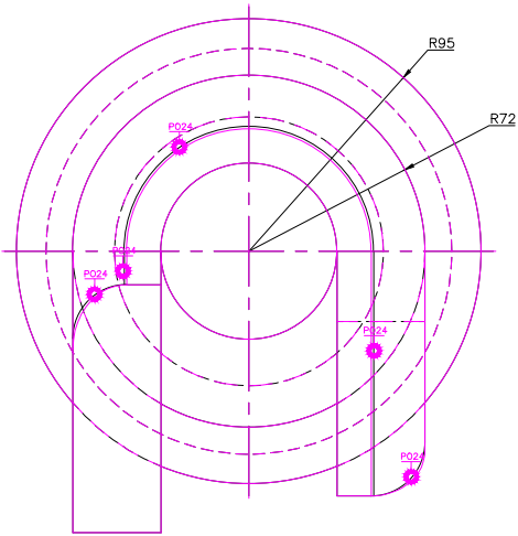
TOP SCALE 1/3
