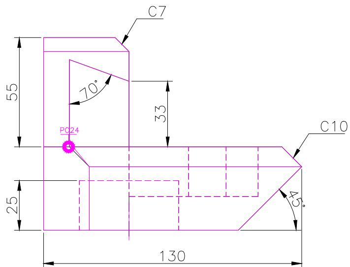
FRONT SCALE 1/2
