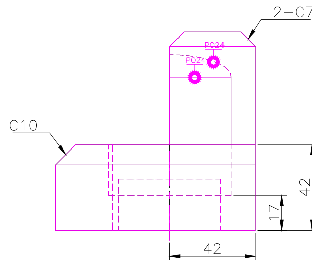
RIGHT SCALE 1/2
