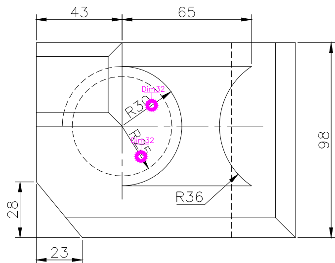
TOP SCALE 1/2
