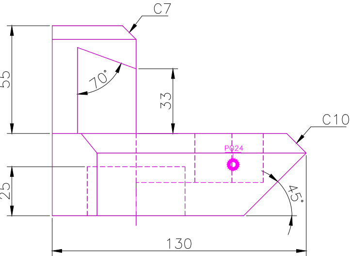
FRONT SCALE 1/2
