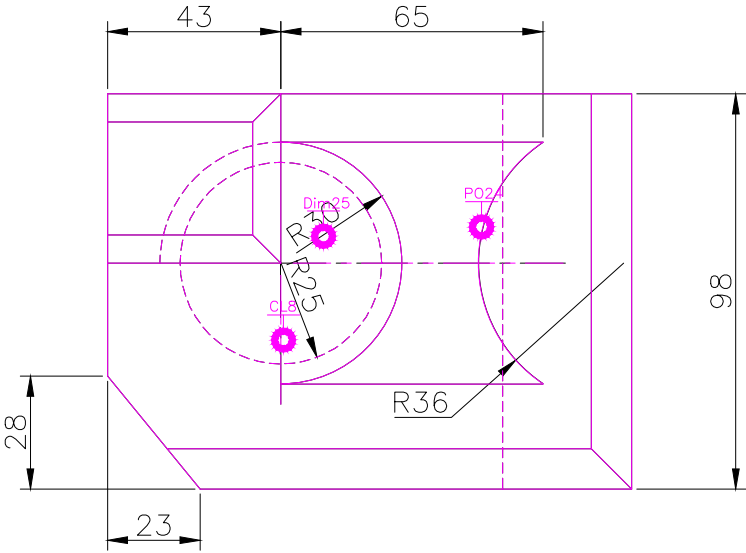
TOP SCALE 1/2
