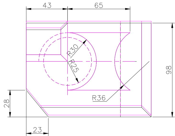
TOP SCALE 1/2
