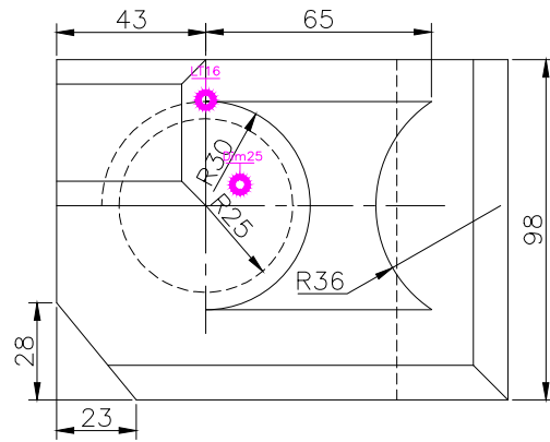
TOP SCALE 1/2
