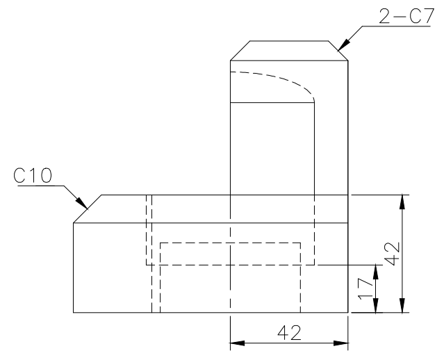
RIGHT SCALE 1/2
