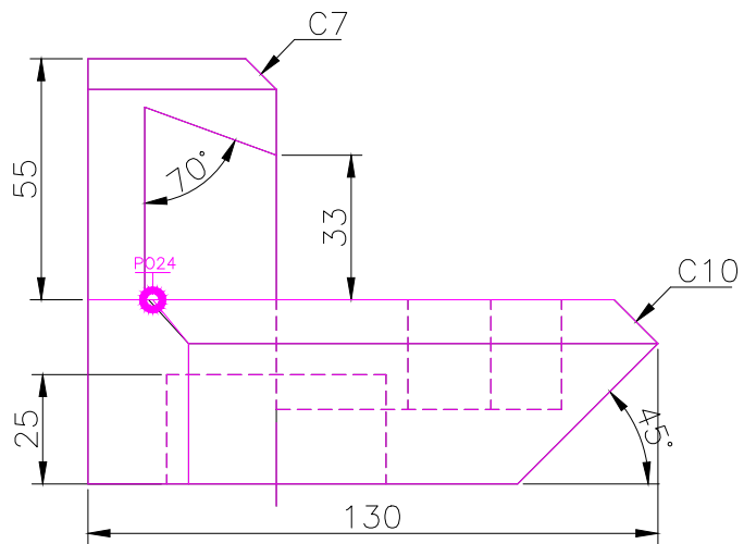
FRONT SCALE 1/2
