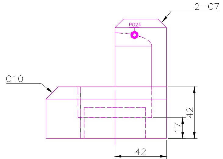
RIGHT SCALE 1/2
