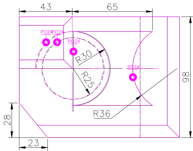
TOP SCALE 1/2
