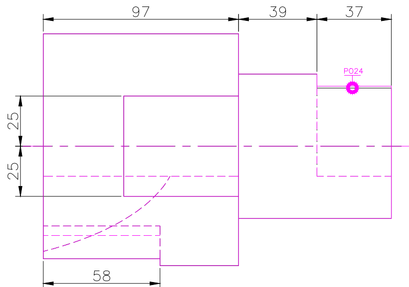
TOP SCALE 1/2
