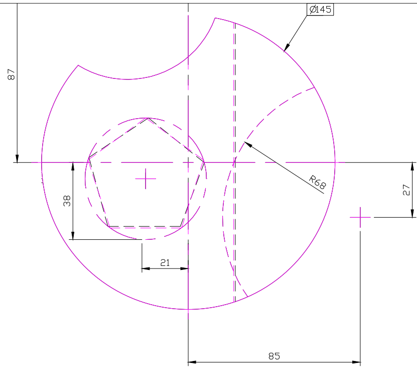
TOP SCALE 1/2
