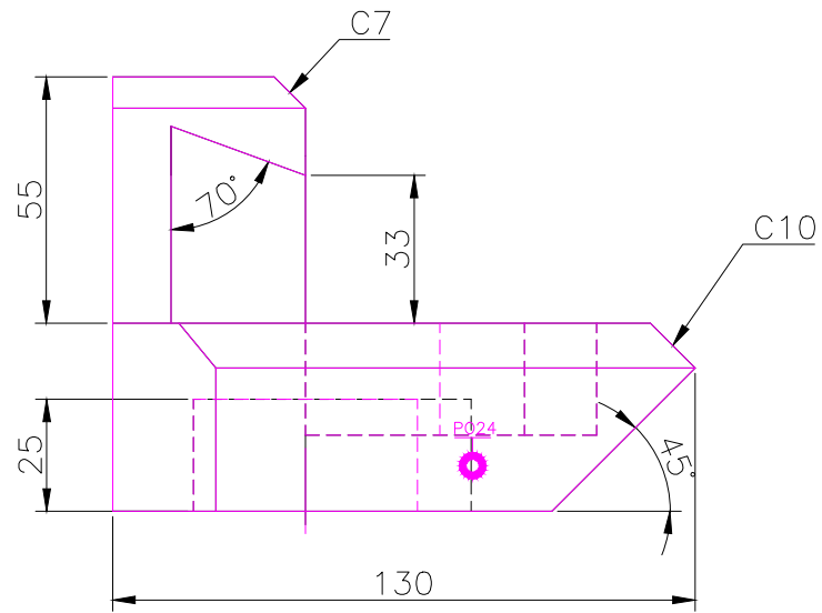
FRONT SCALE 1/2
