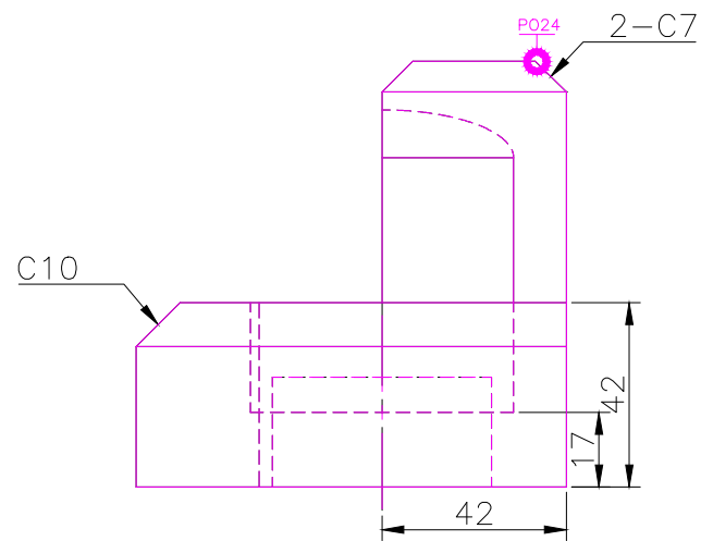
RIGHT SCALE 1/2
