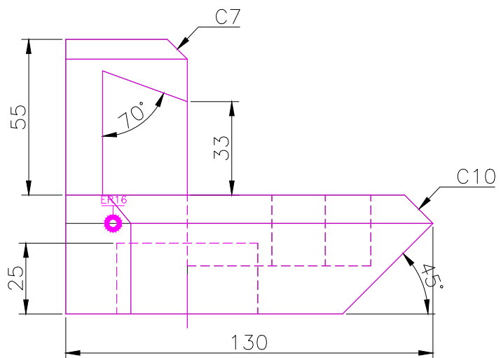
FRONT SCALE 1/2
