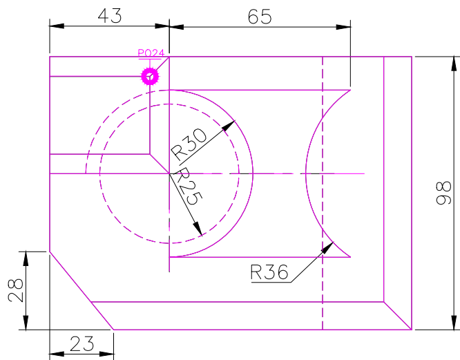
TOP SCALE 1/2
