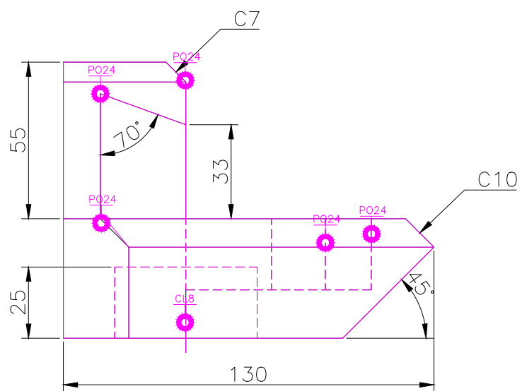
FRONT SCALE 1/2
