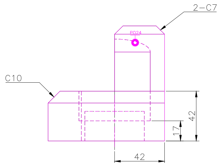
RIGHT SCALE 1/2
