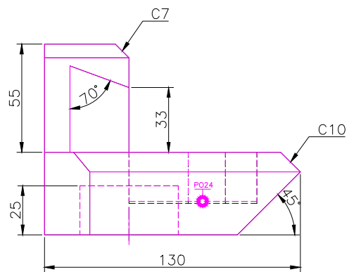
FRONT SCALE 1/2
