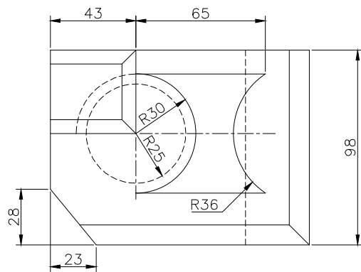
TOP SCALE 1/2
