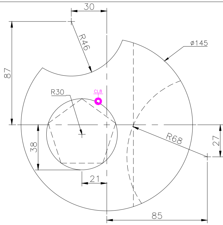
TOP SCALE 1/2
