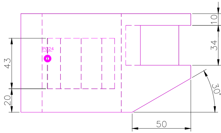
FRONT SCALE 1/2
