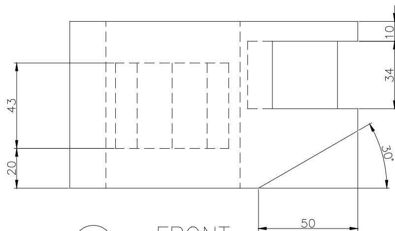
FRONT SCALE 1/2
