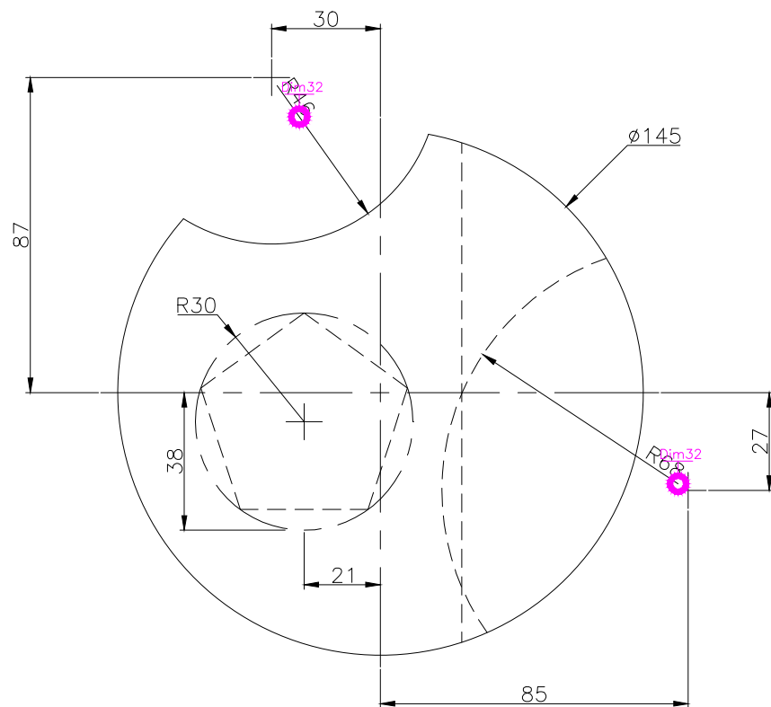
TOP SCALE 1/2
