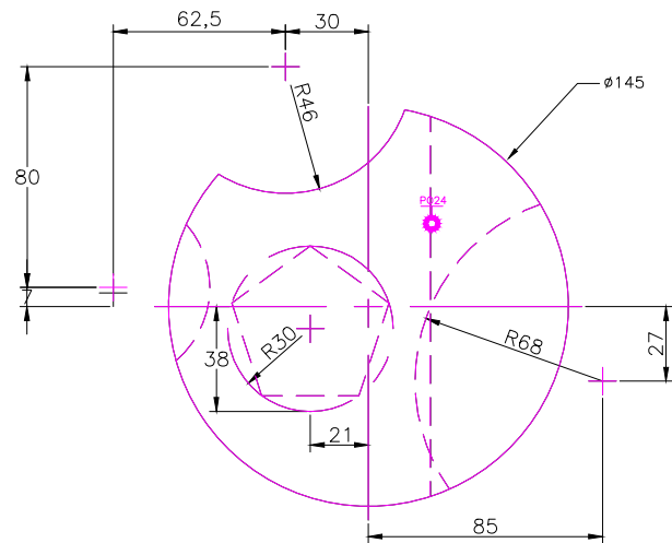
TOP SCALE 1/2
