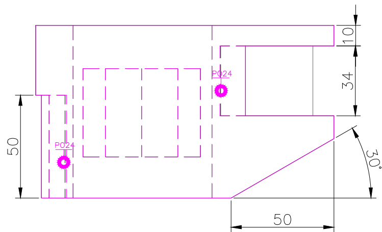
FRONT SCALE 1/2
