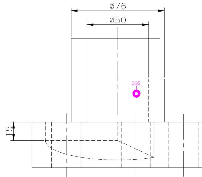
RIGHT SCALE 1/2
