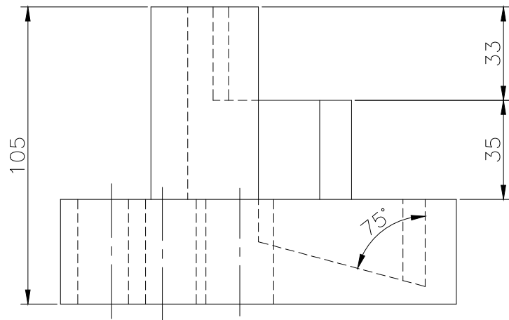
FRONT SCALE 1/2
