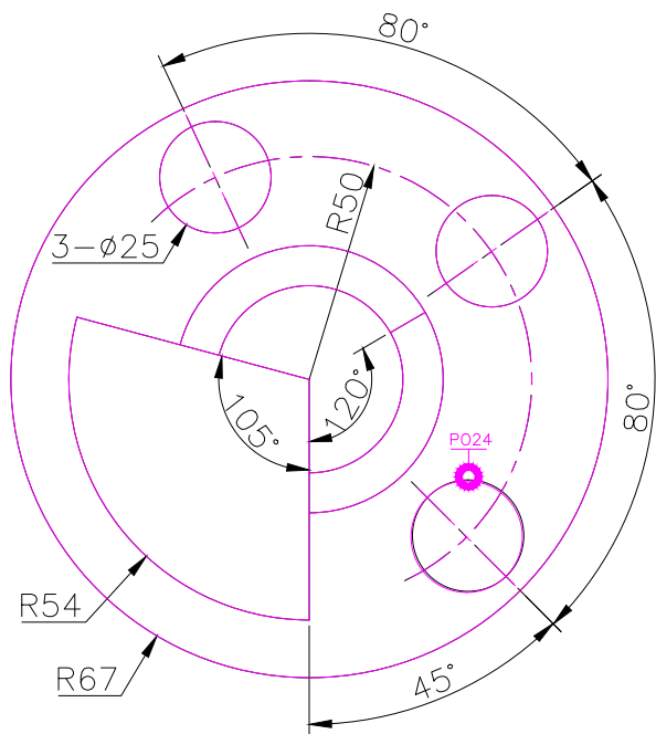
TOP SCALE 1/2
