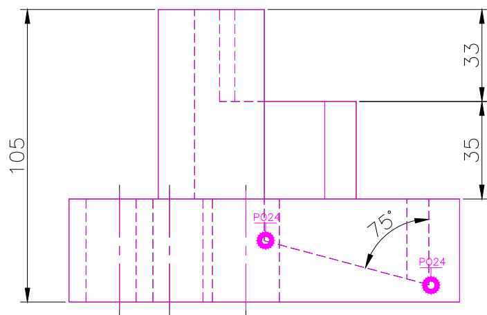
FRONT SCALE 1/2
