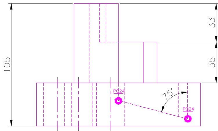
FRONT SCALE 1/2
