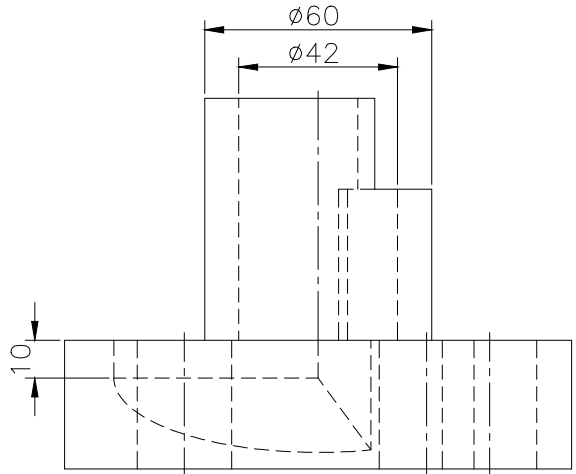
RIGHT SCALE 1/2
