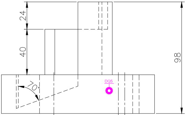
FRONT SCALE 1/2
