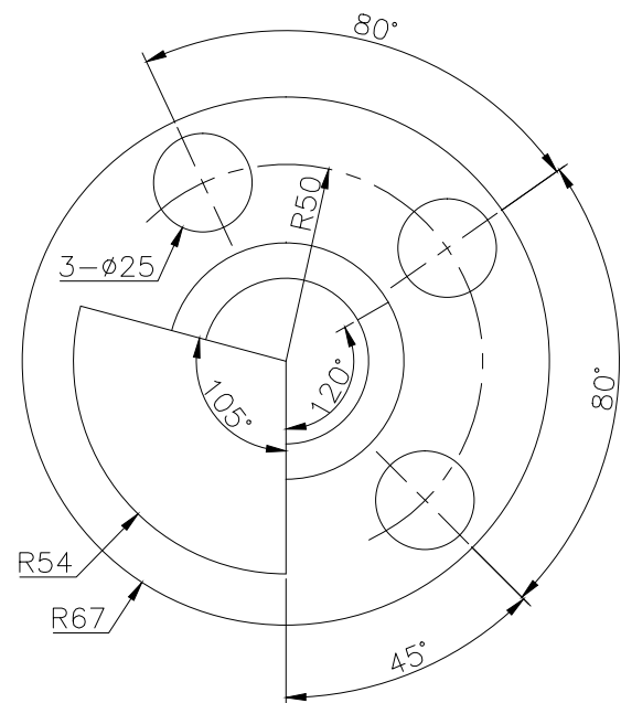
TOP SCALE 1/2
