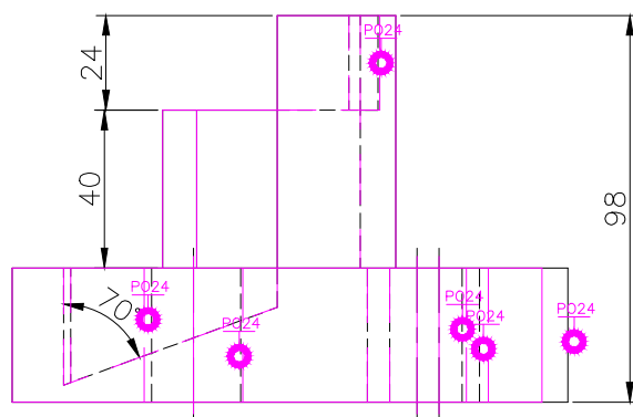
FRONT SCALE 1/2
