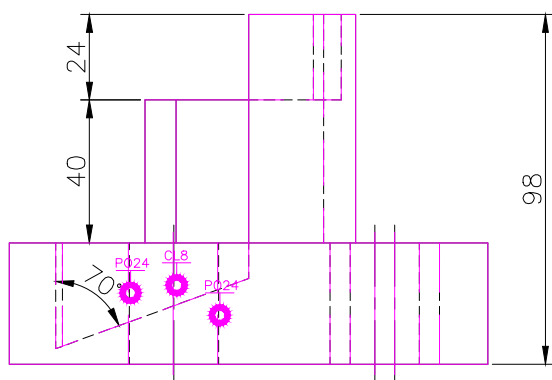
FRONT SCALE 1/2
