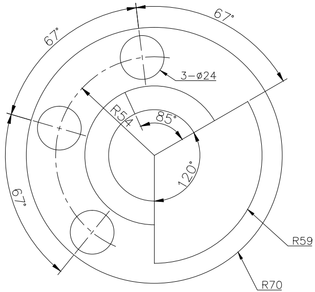
TOP SCALE 1/2
