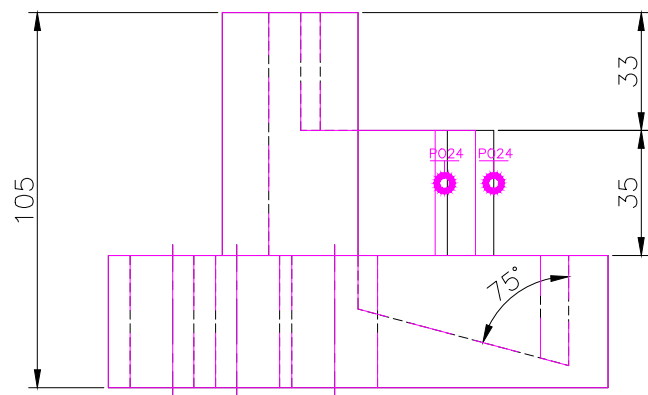
FRONT SCALE 1/2
