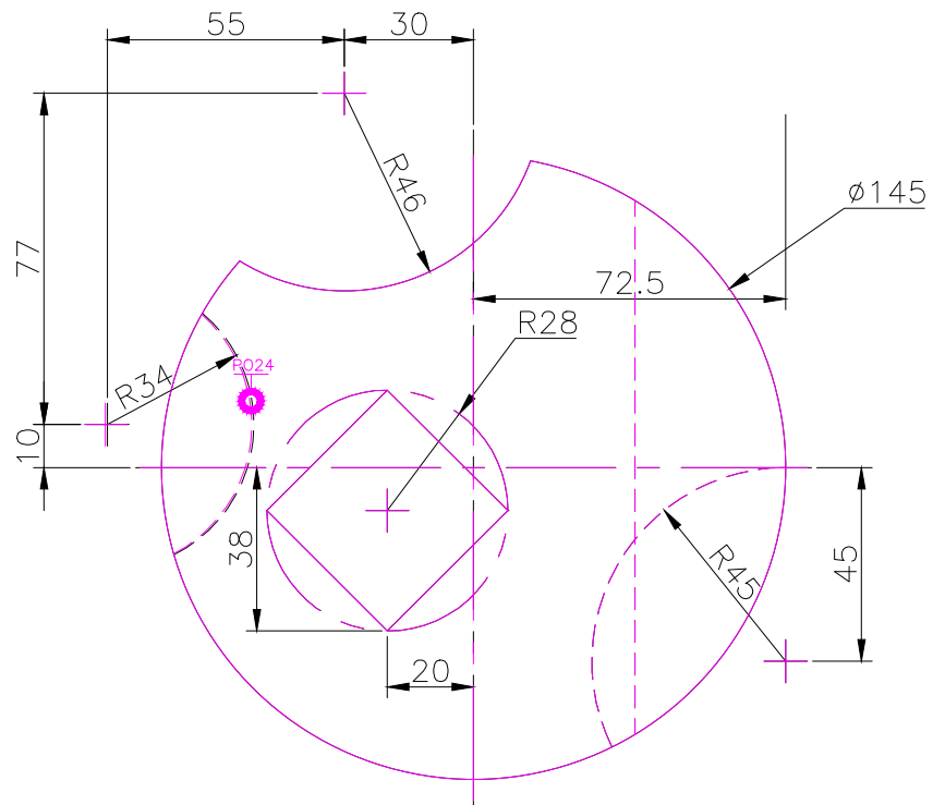
TOP SCALE 1/2
