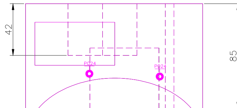
RIGHT SCALE 1/2
