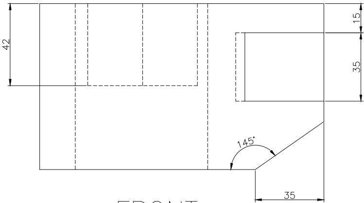
FRONT SCALE 1/2
