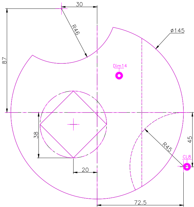
TOP SCALE 1/2
