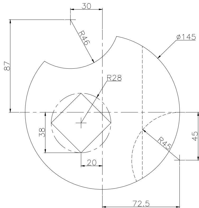
TOP SCALE 1/2
