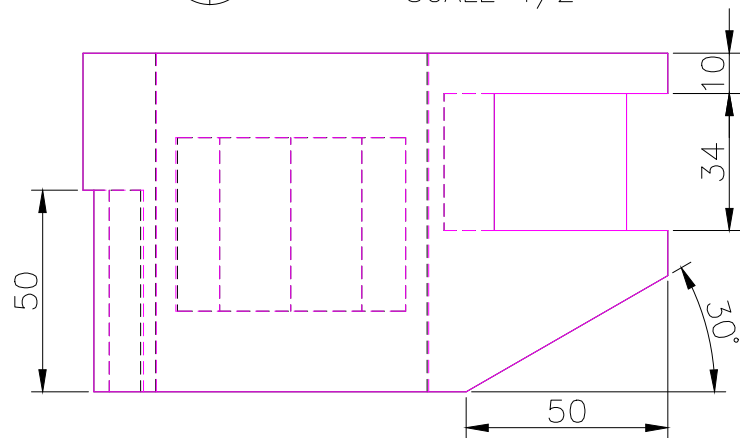
FRONT SCALE 1/2
