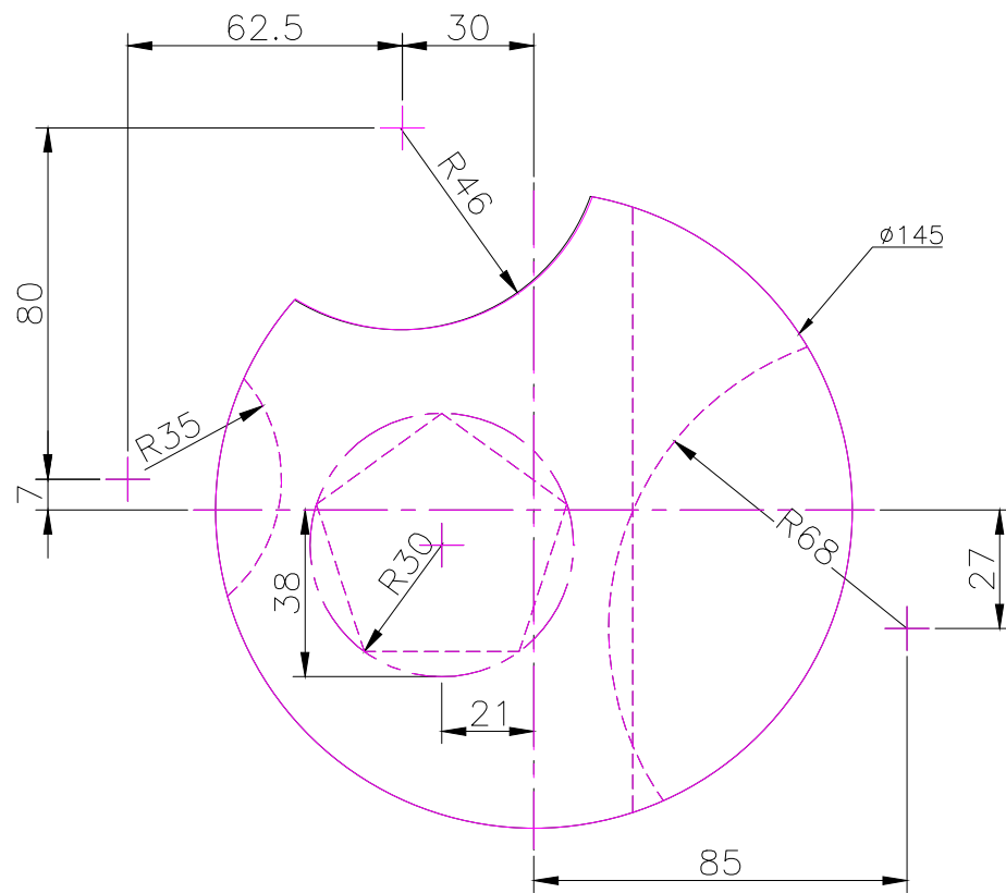
TOP SCALE 1/2
