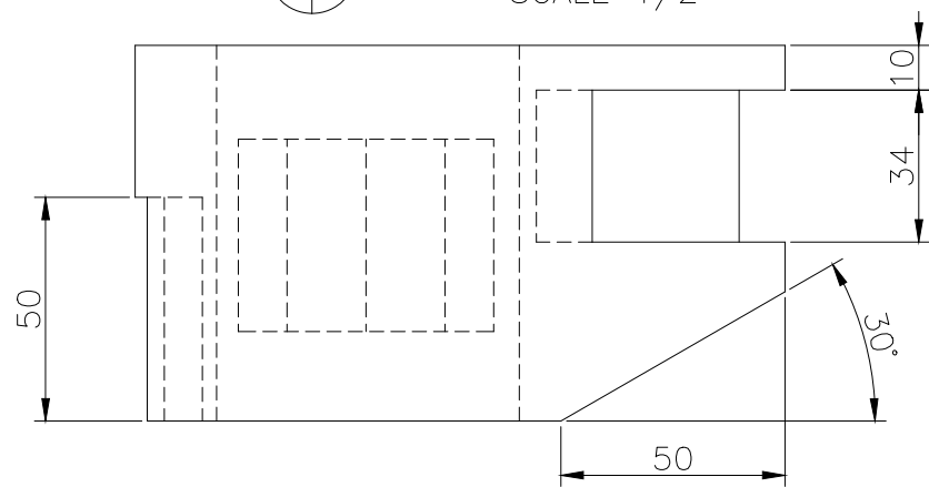
FRONT SCALE 1/2
