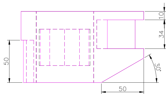
FRONT SCALE 1/2
