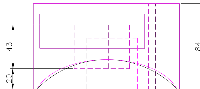
RIGHT SCALE 1/2
