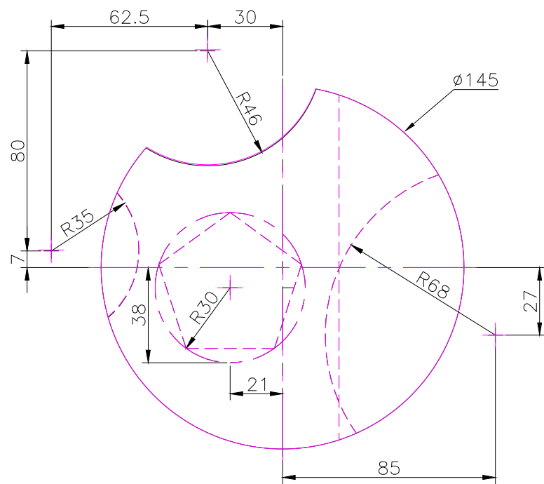
TOP SCALE 1/2
