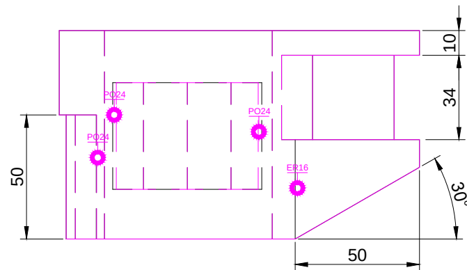
FRONT SCALE 1/2
