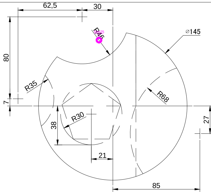
TOP SCALE 1/2
