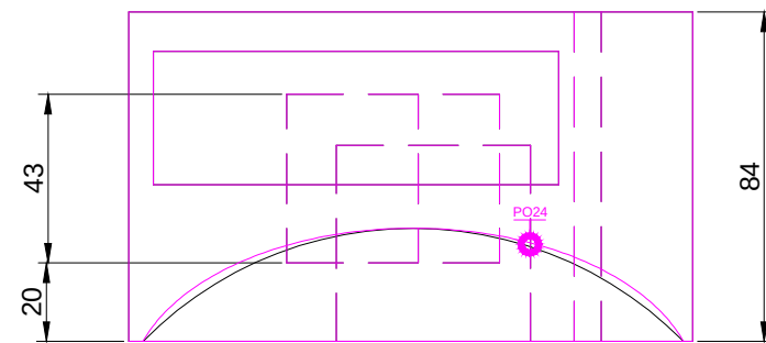
RIGHT SCALE 1/2
