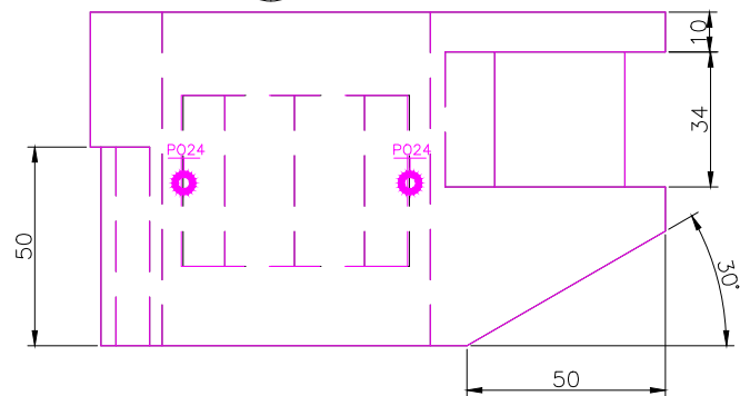
FRONT SCALE 1/2
