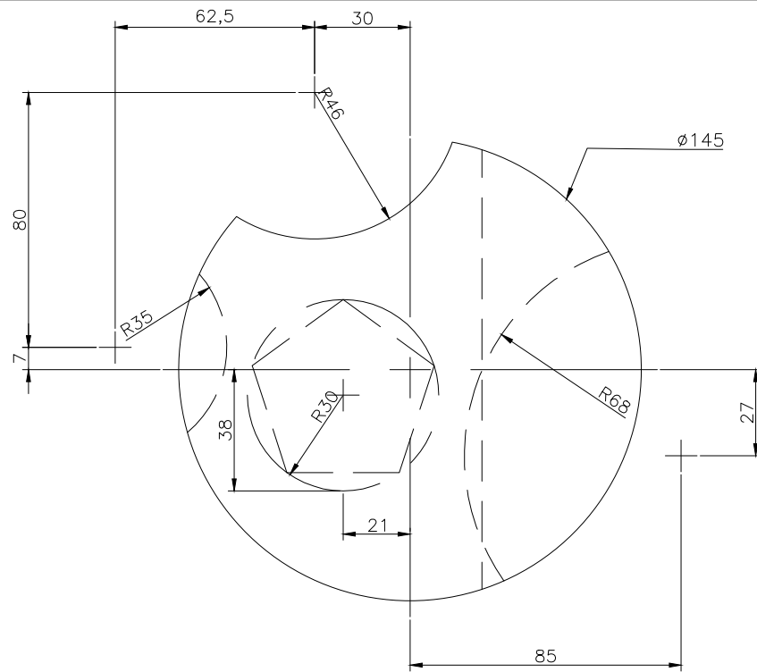
TOP SCALE 1/2
