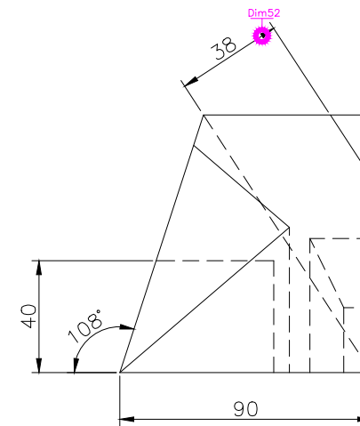
RIGHT SCALE 1/2
